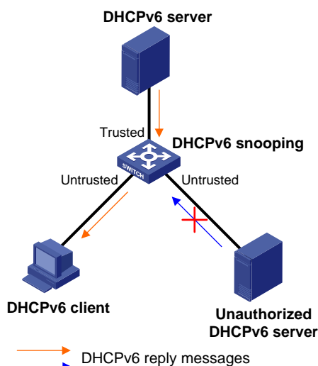
Figure 70 Trusted and untrusted ports
